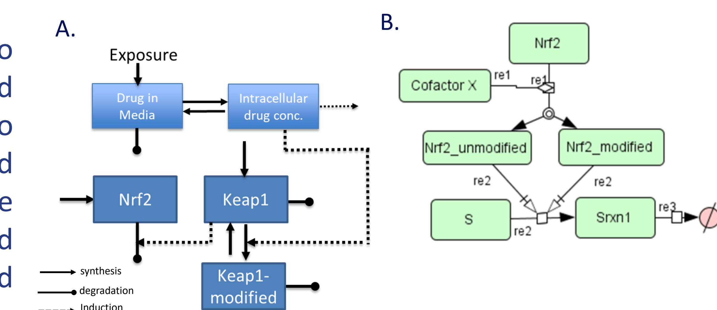
Fig 1: Modeling strategy to describe chemical kinetics and Nrf2 dynamics (A), and Srxn1 dynamics (B). C) Fitting strategy with non-linear mixed-effects modelling. Abbr. Nrf2 – (Nuclear factor erythroid 2-related factor 2), Srxn1- (Sulfiredoxin-1), Keap1- (Kelch-like ECH-associated protein 1), S-(Substrate), CofactorX –(a hypothetical set of Nrf2 modifiers)
